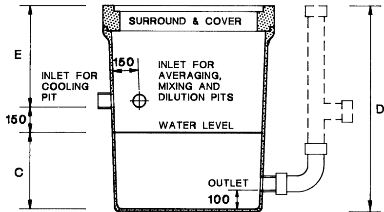
SECTION
