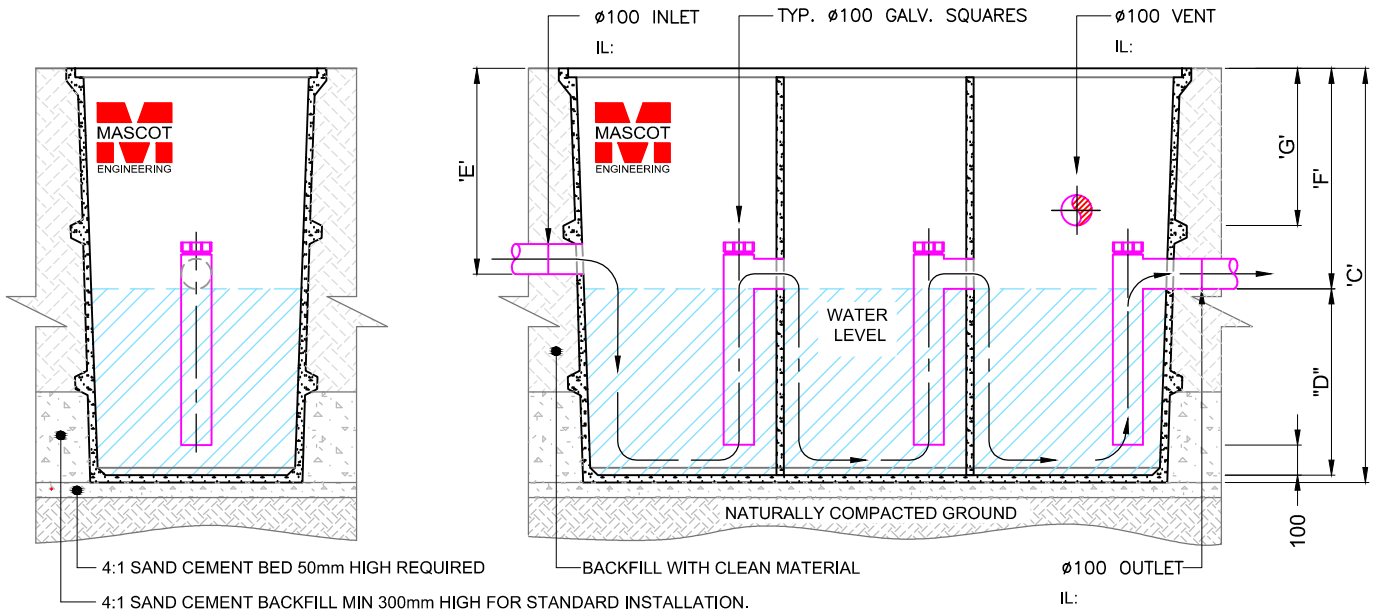
END SECTION SCALE 1:25
