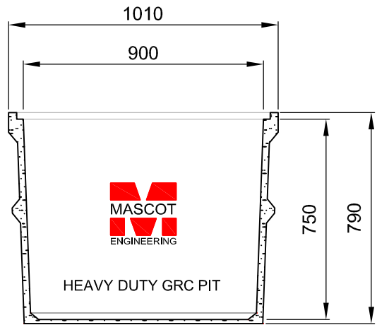
SECTION VIEW
