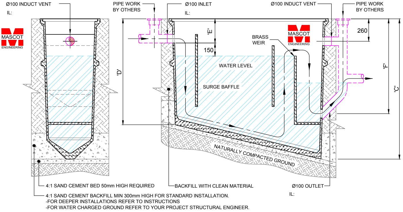
END SECTION SCALE 1:25
