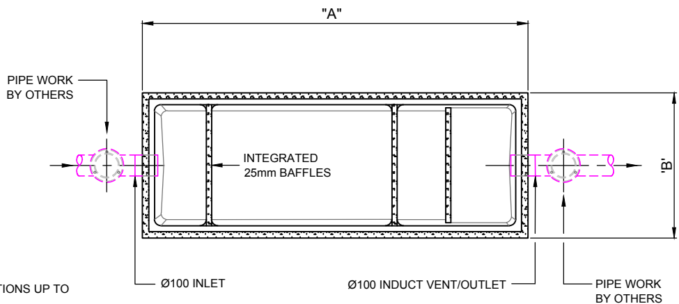
OPEN TANK PLAN VIEW SCALE 1:25
