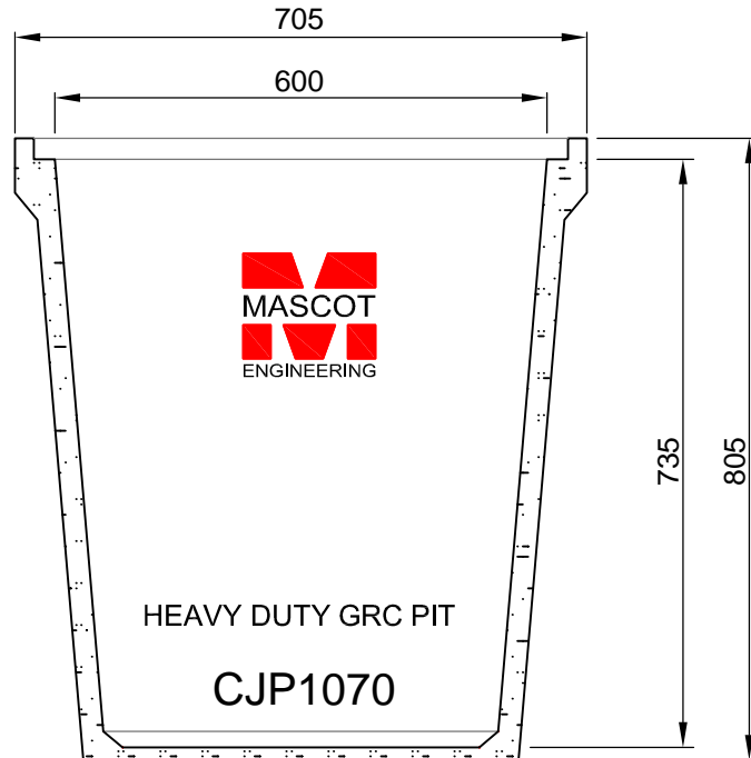
SECTION VIEW
