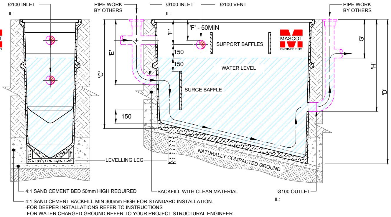
END SECTION SCALE 1:25
