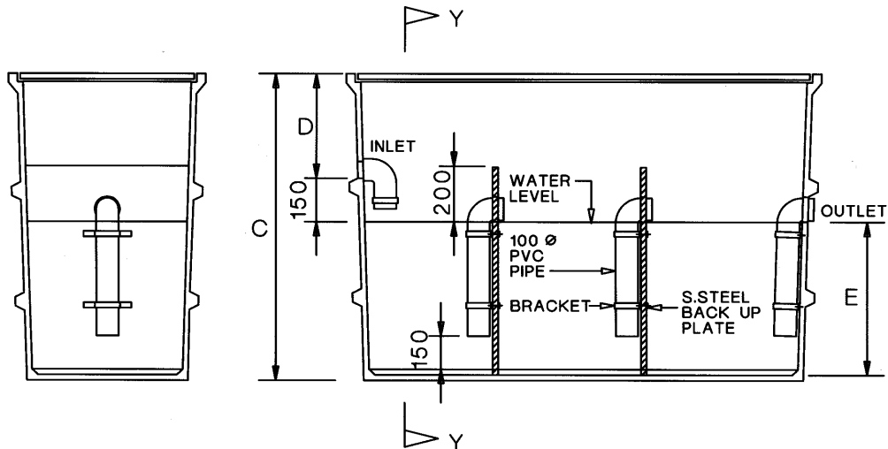
SECTION Y-Y
